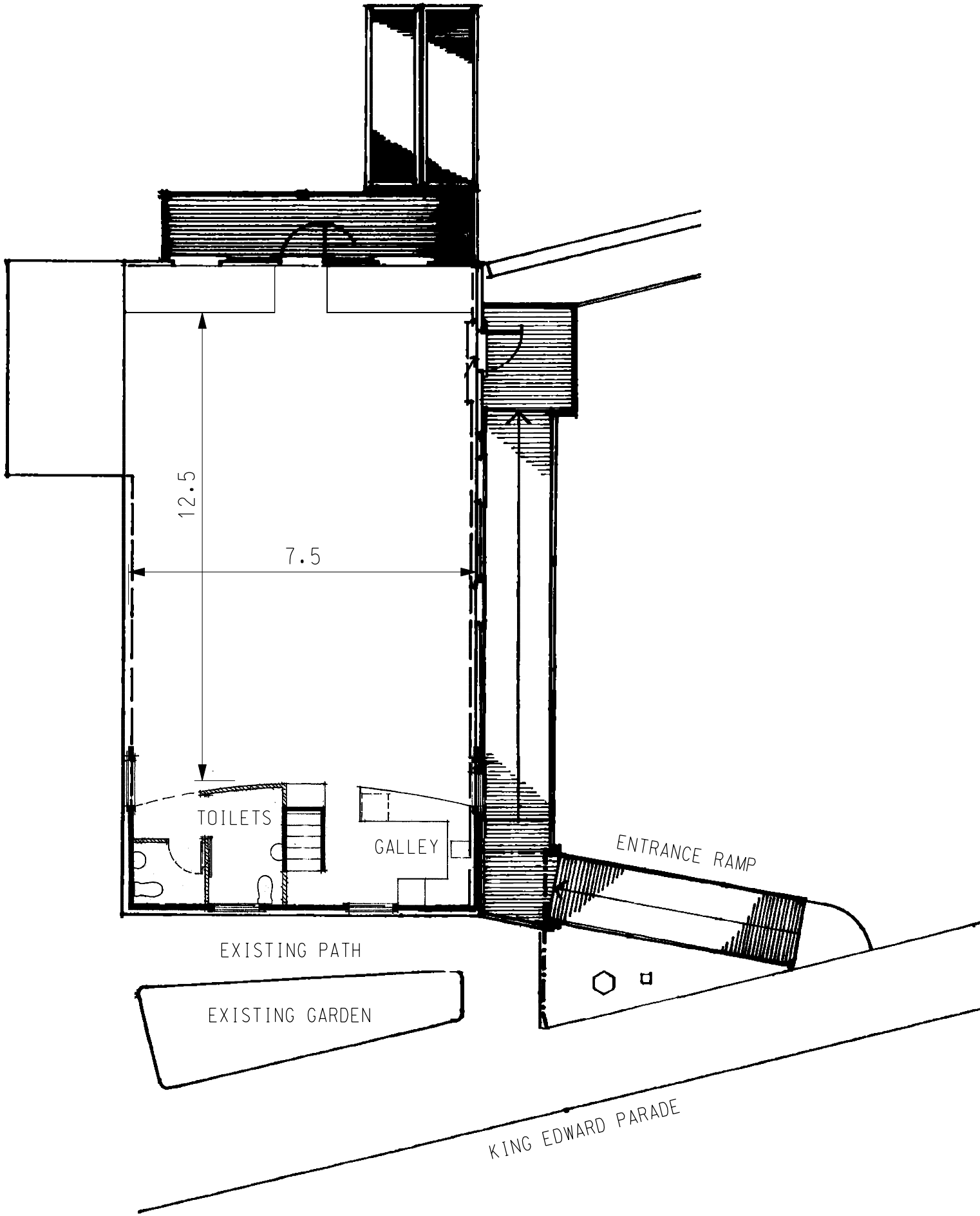
INTERNAL LAYOUT
